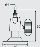
Mount Bracket
